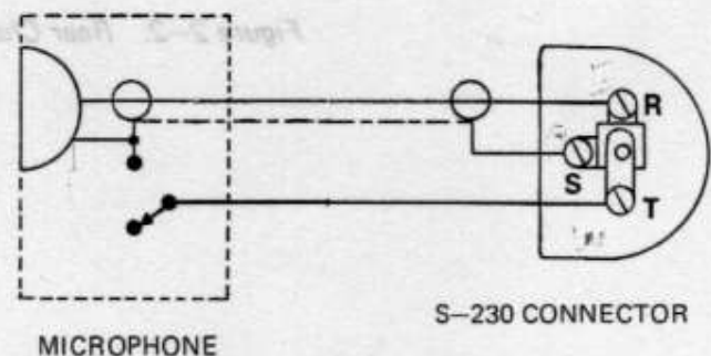
Figure 2-1. Microphone Connections
