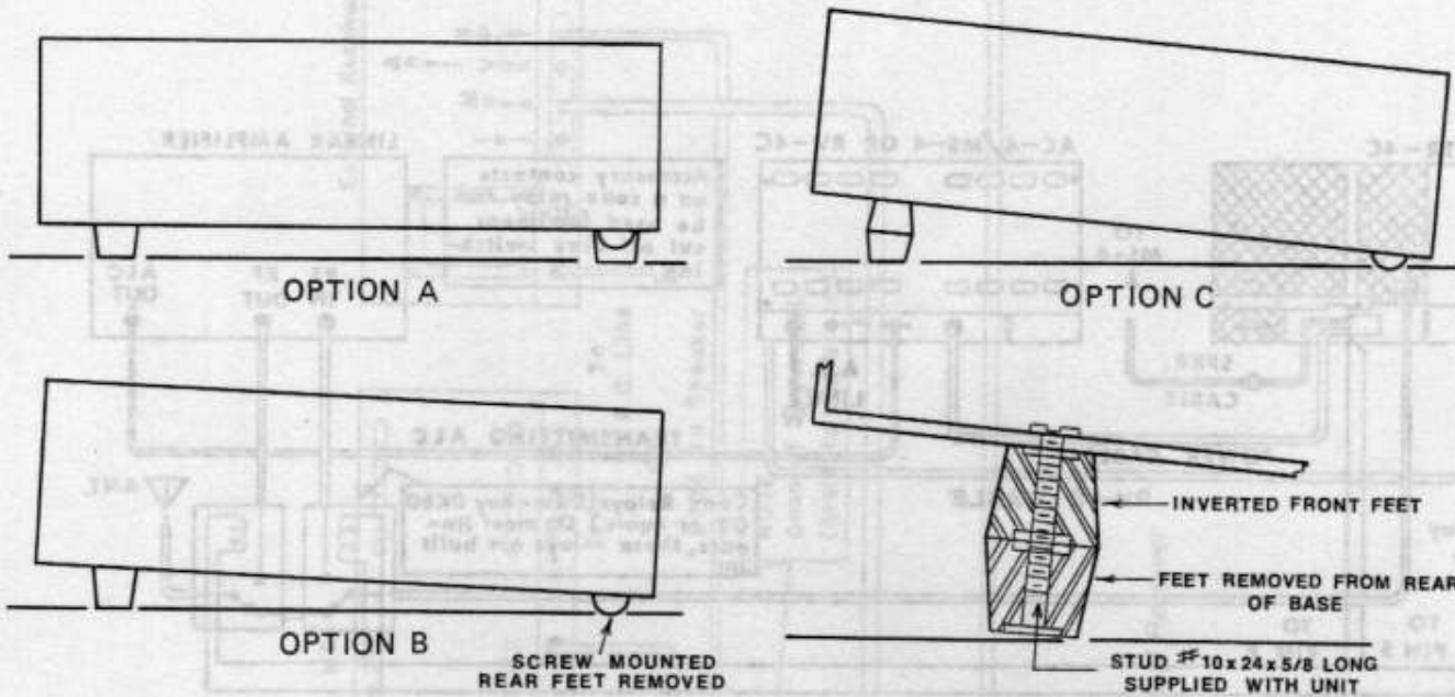
Figure 2-5. Viewing Angle Options in a Stationary Installation
