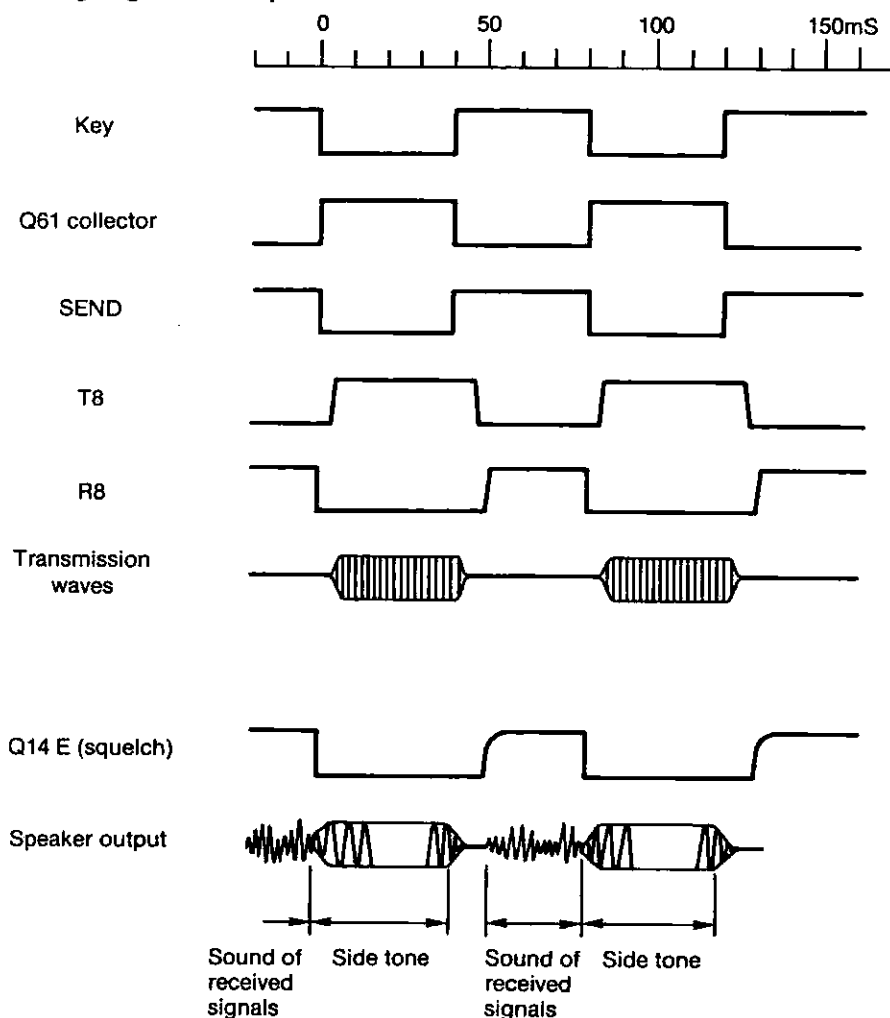
Timing diagram of CW operation
