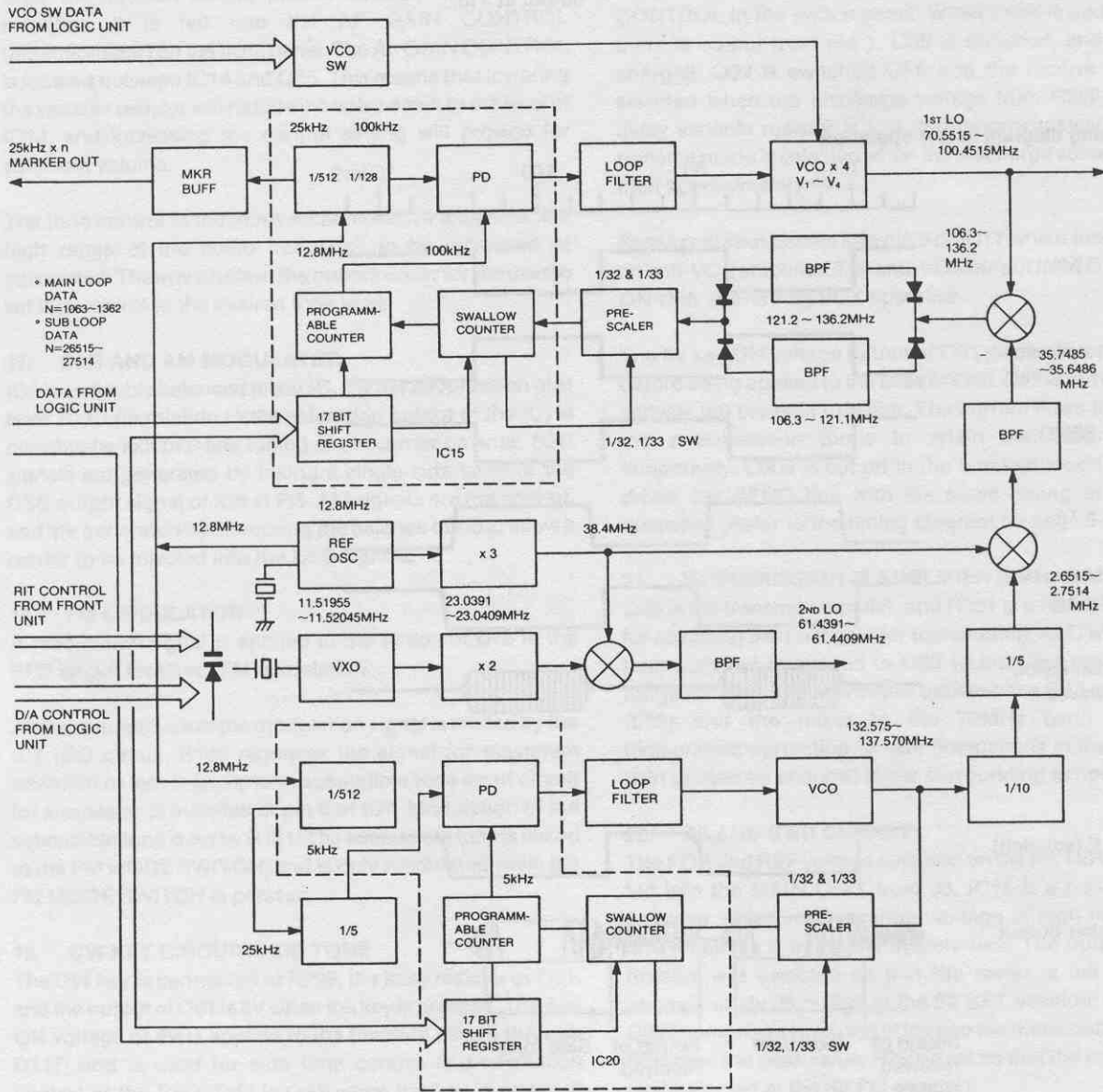
PLL block diagram
