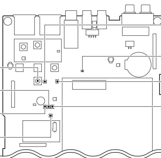
Bottom view of the transceiver
