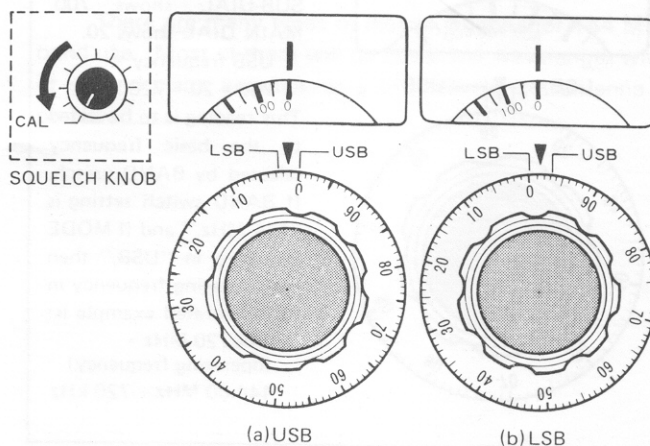
Fig. 9 Frequency Calibration
