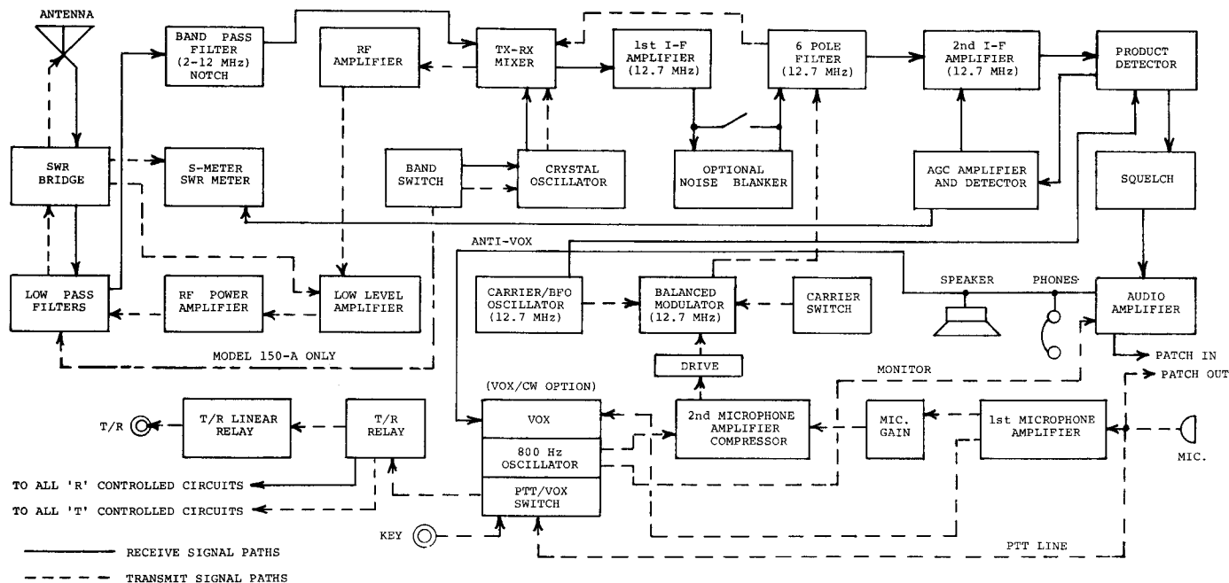
Figure 7 - Block Diagram
