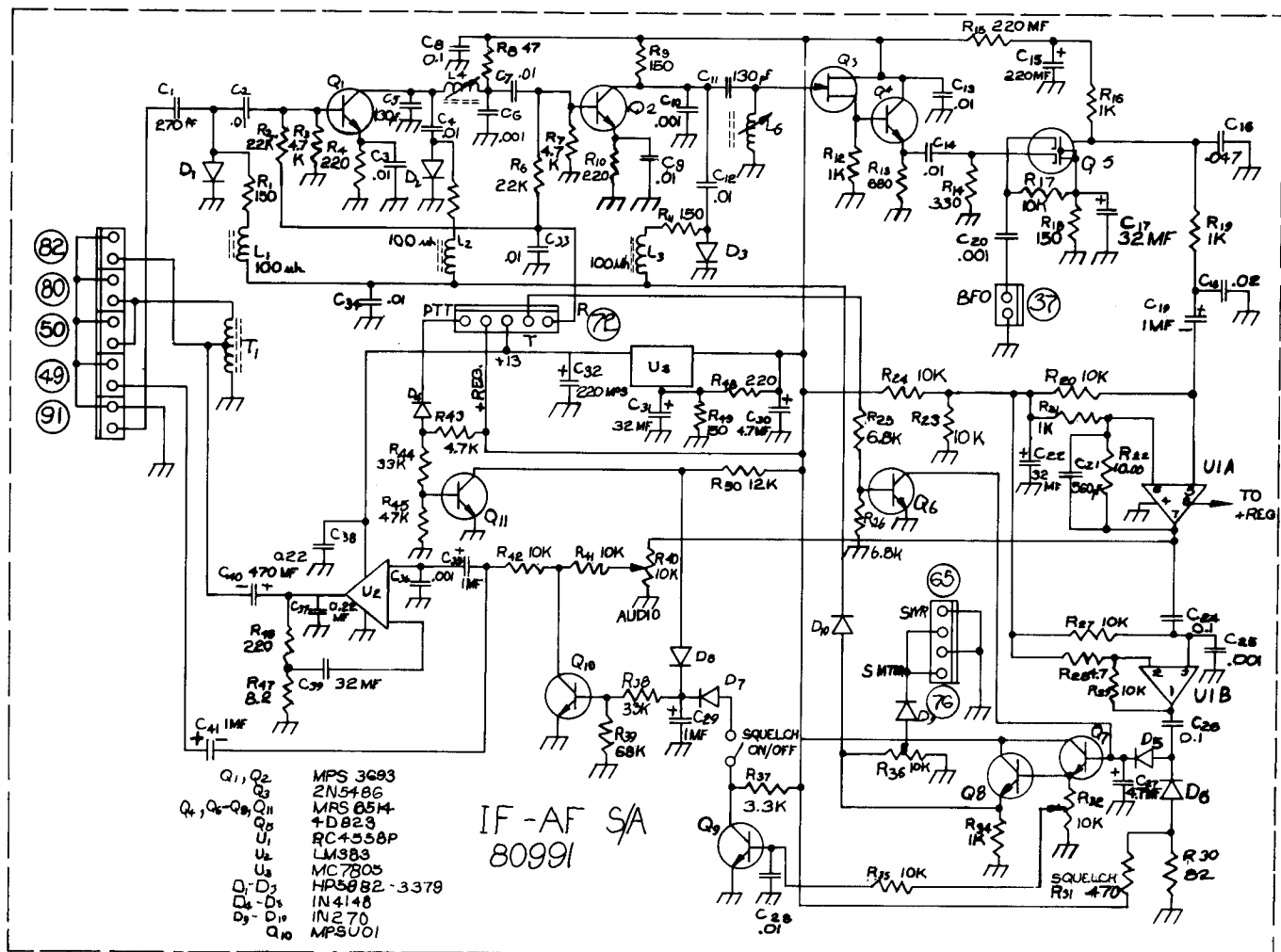
IF/AF Schematic
