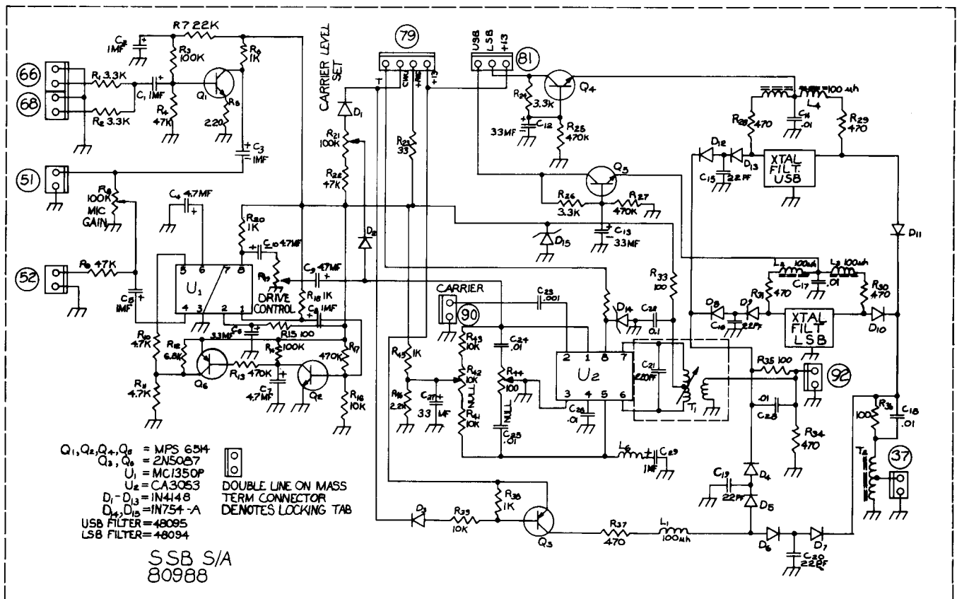
SSB Schematic
