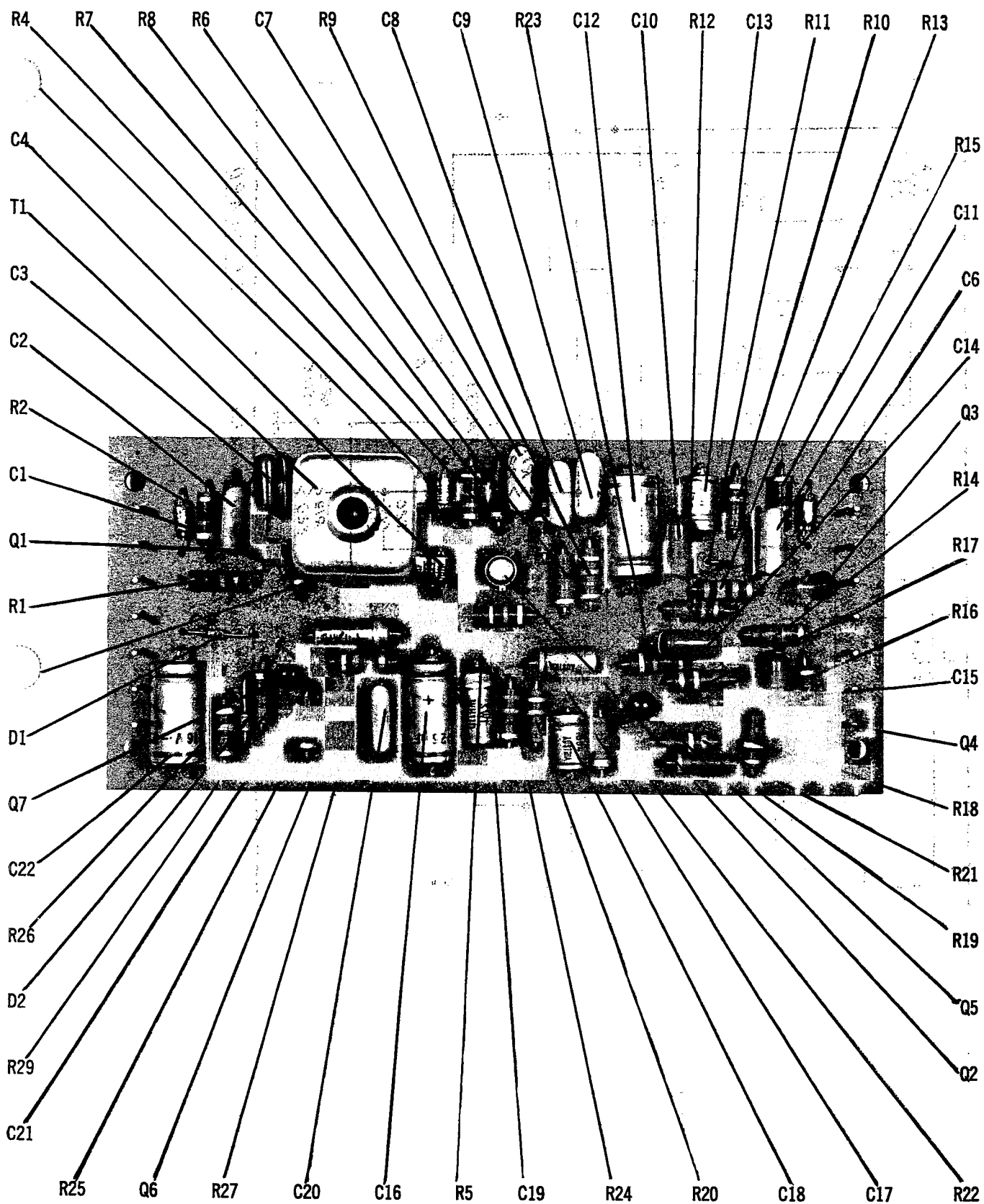
90184 IF BOARD
