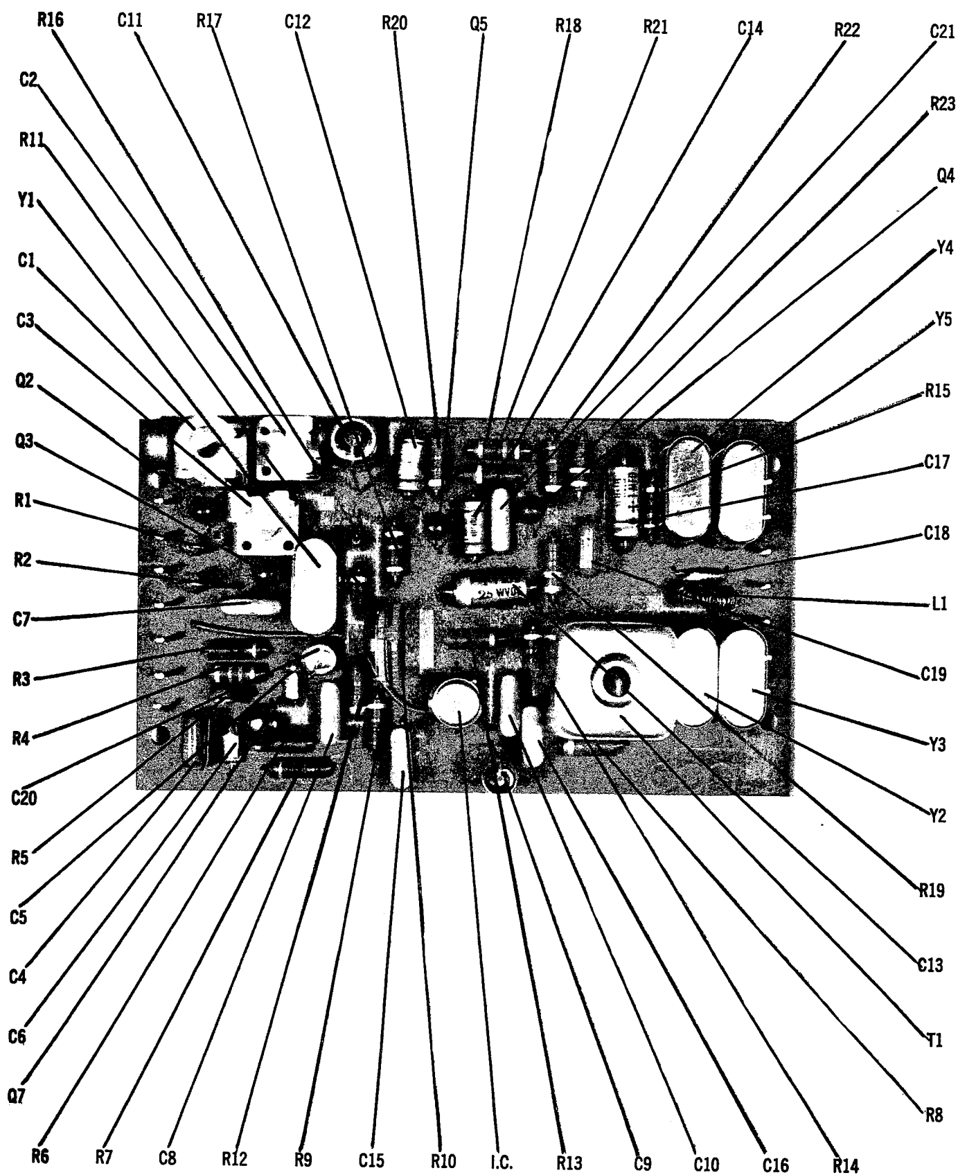
90191 SSB GENERATOR
