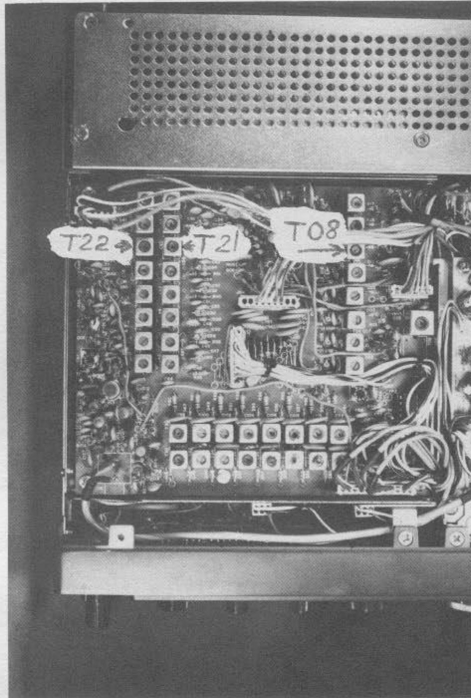
RF board
