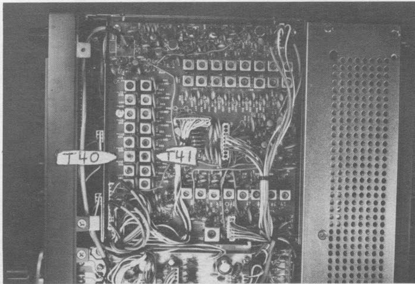
Rf board
