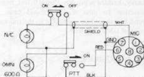
YM-36 MICROPHONE CONNECTIONS
