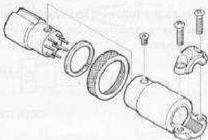
YM-37 MICROPHONE CONNECTIONS
